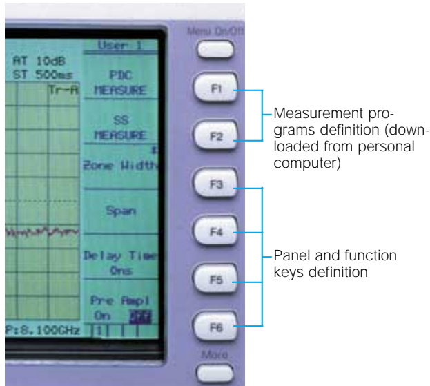
User-defined menu
