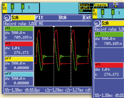
Wave forms of current and voltage
